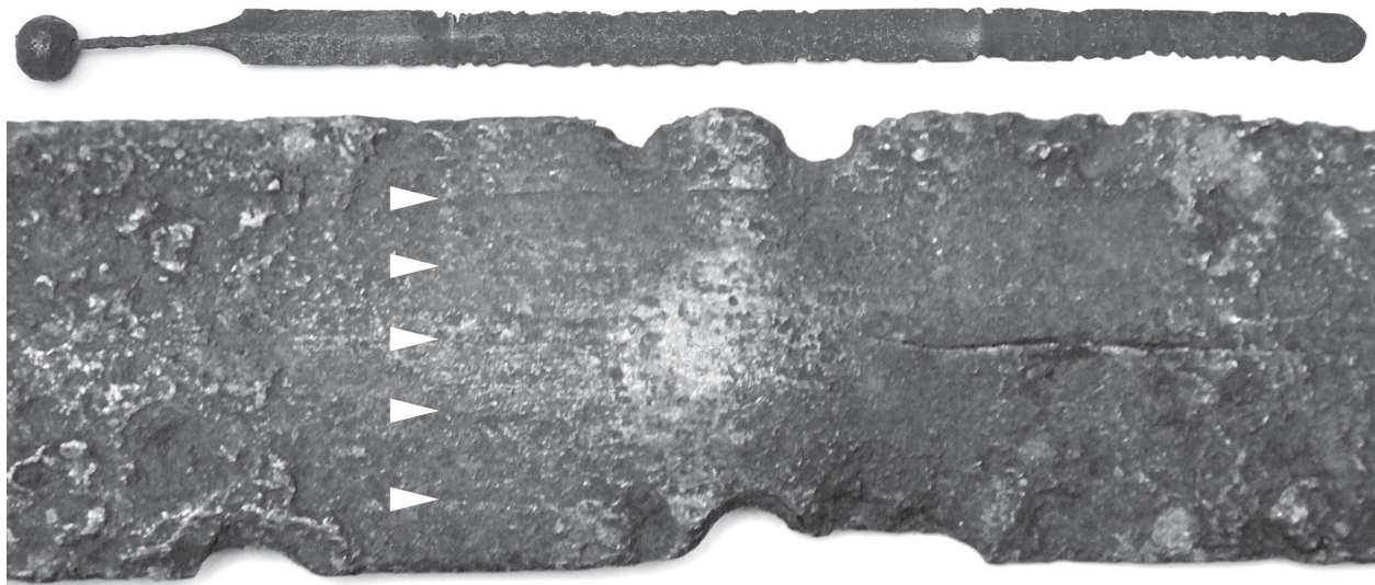
Celtic sword from the 1st century BC, in an area presumably bent prior to inhumation and later straightened. Differential corrosion discloses separate elements for each cutting edge and linearity parallel to the long axis suggests four additional elements in this piled construct (white arrows denote weld boundaries). A parallel stress fracture is seen to the right and appears to be along a welded boundary.
